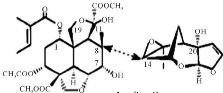
Azadiractina
